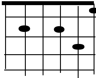
X 2 X 3 4 1
