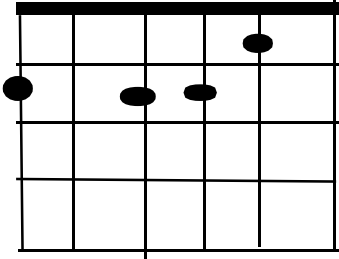
2 X 3 4 1 X
