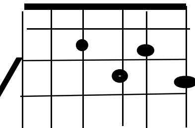
X X 1 3 2 4
